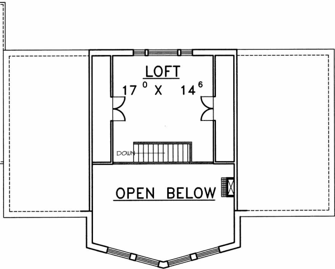
LOFT FLOOR PLAN
