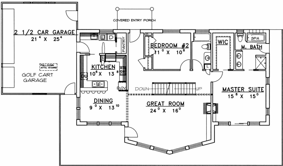
MAIN LEVEL FLOOR PLAN
