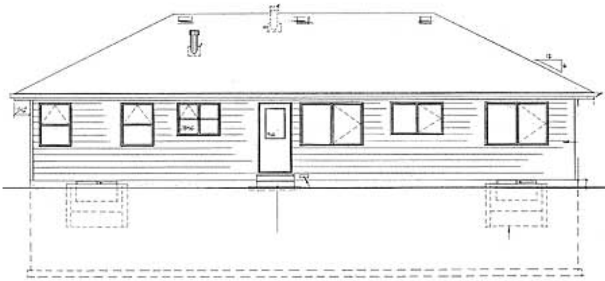
REAR ELEVATION
