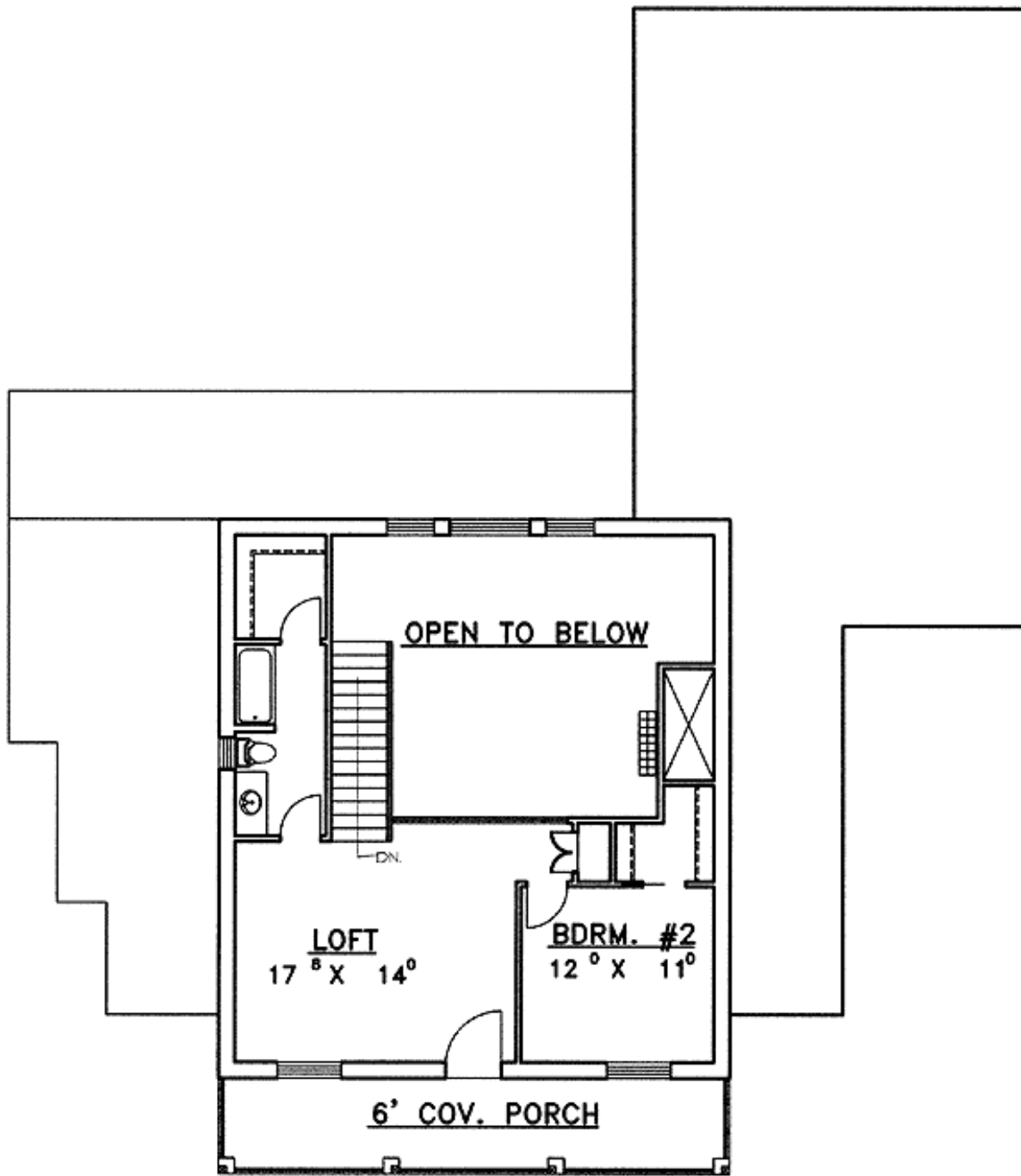
UPPER LEVEL FLOOR PLAN
