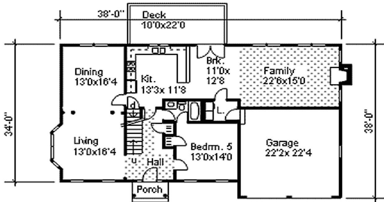
Main Level
