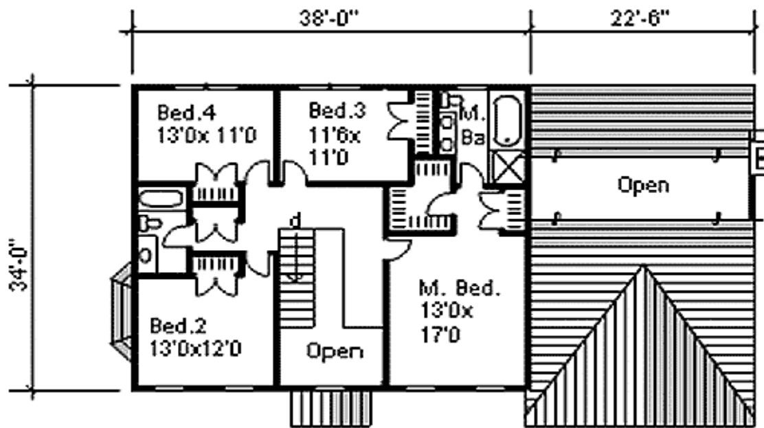
2nd Level
