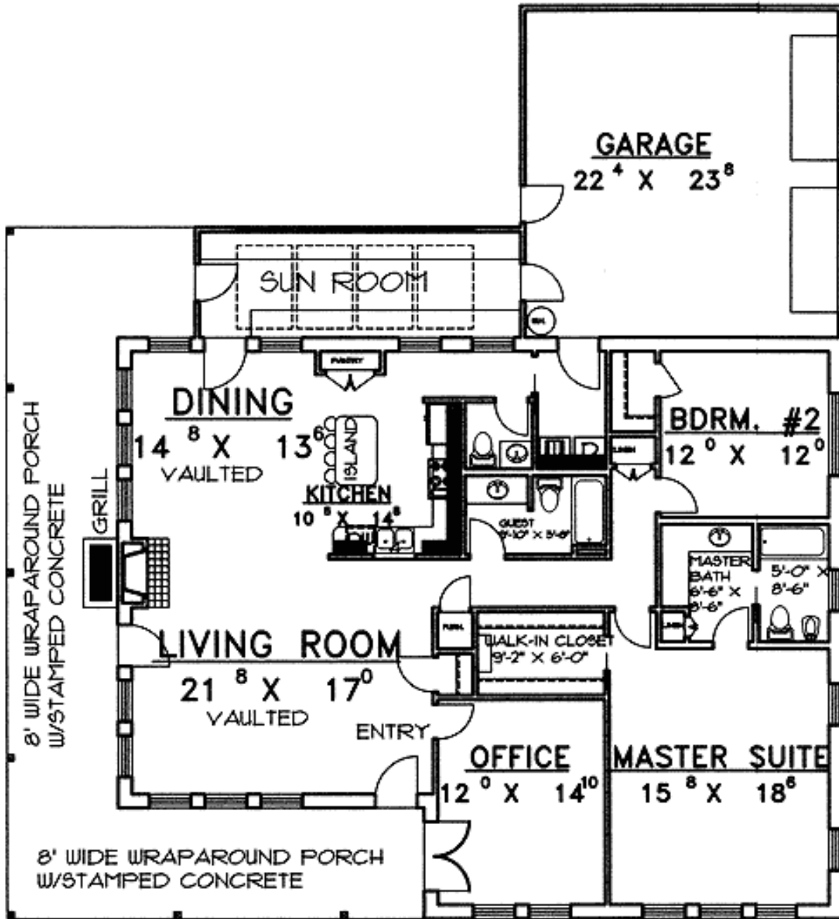
FLOOR PLAN
