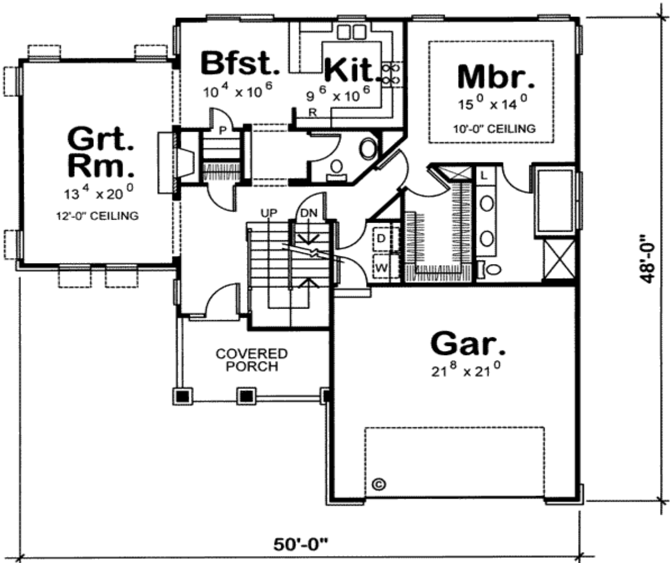
Main Level
