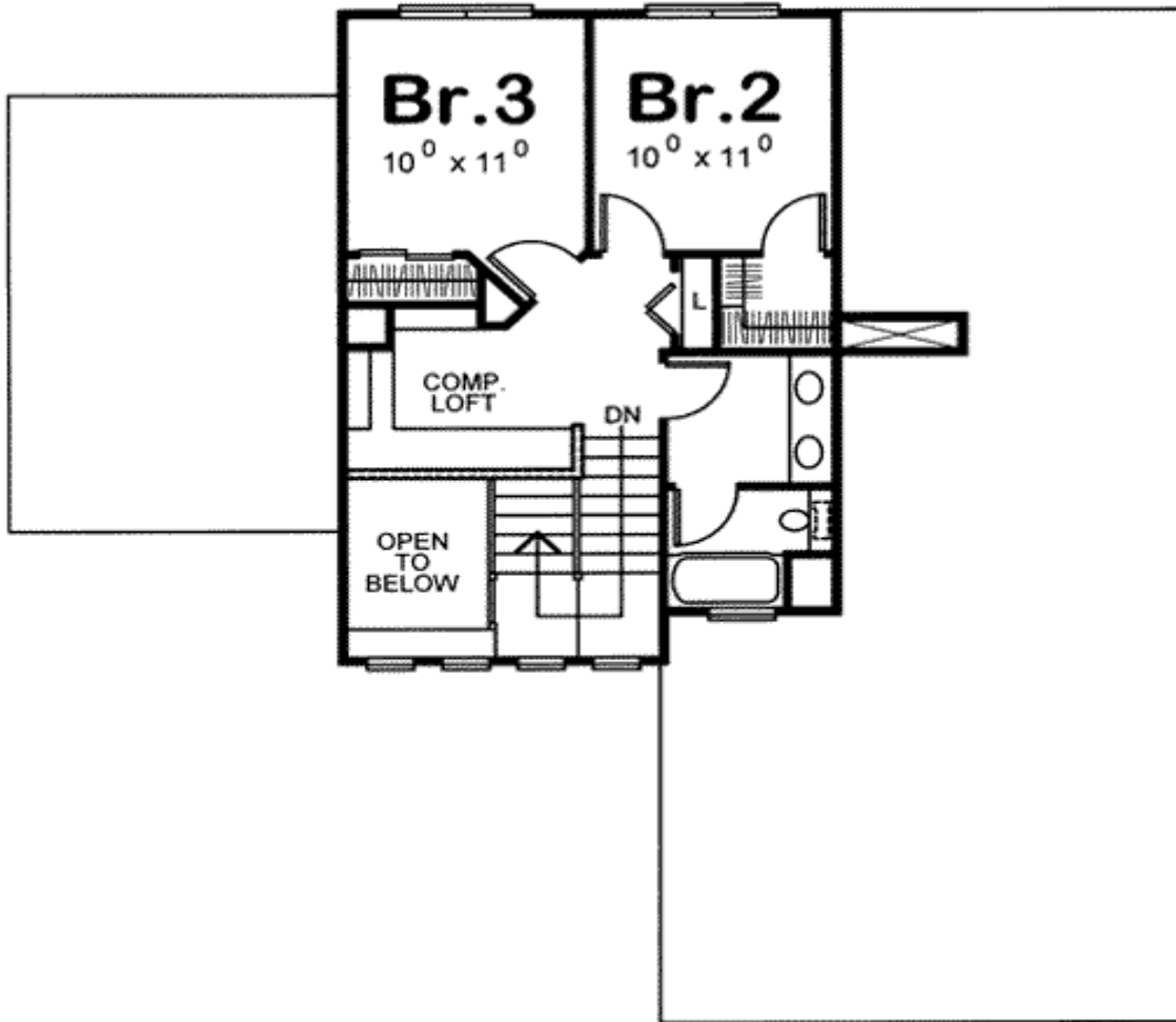
2nd Level
