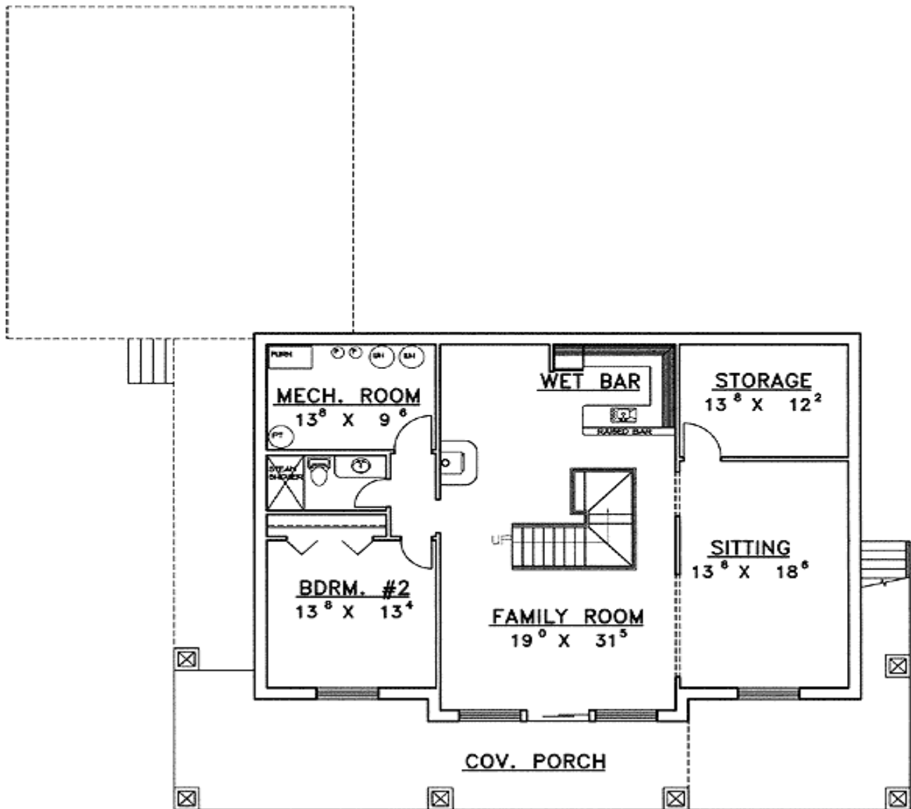
DAYLIGHT BASEMENT PLAN
