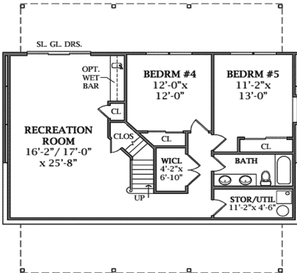
Optional walkout basement plan
