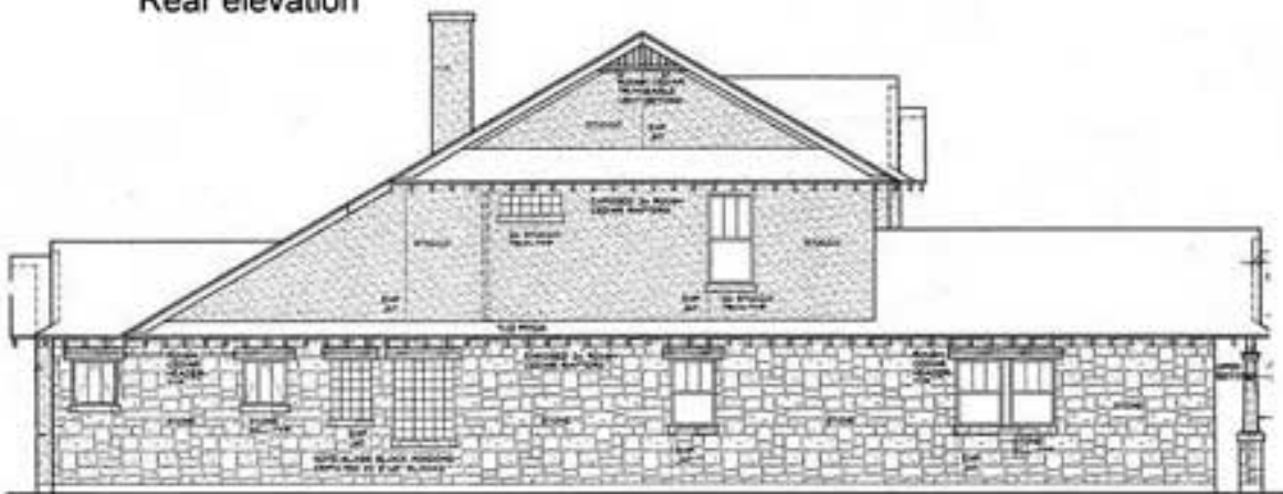
Left elevation
