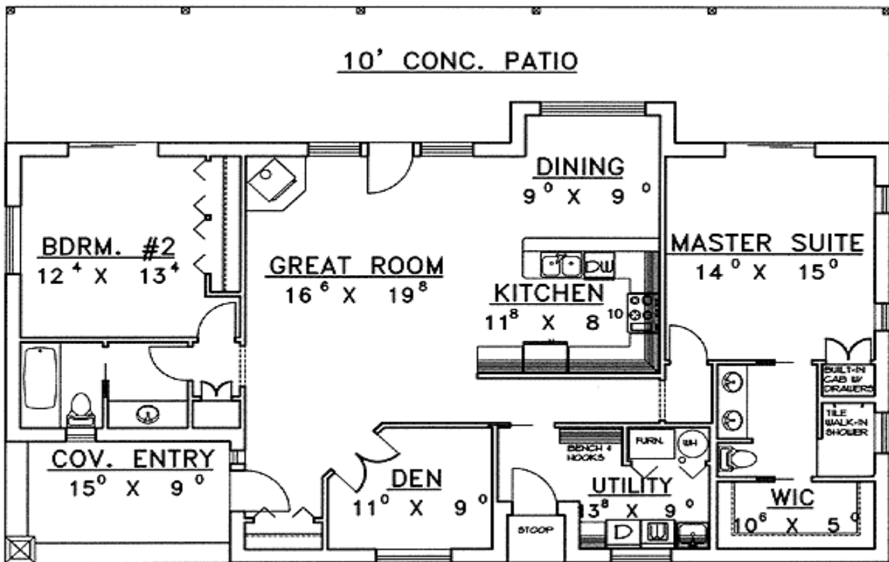
MAIN LEVEL FLOOR PLAN 1721 SQ'
