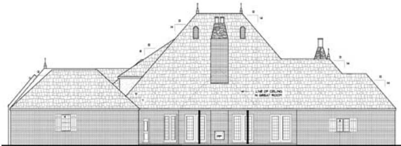
REAR ELEVATION
