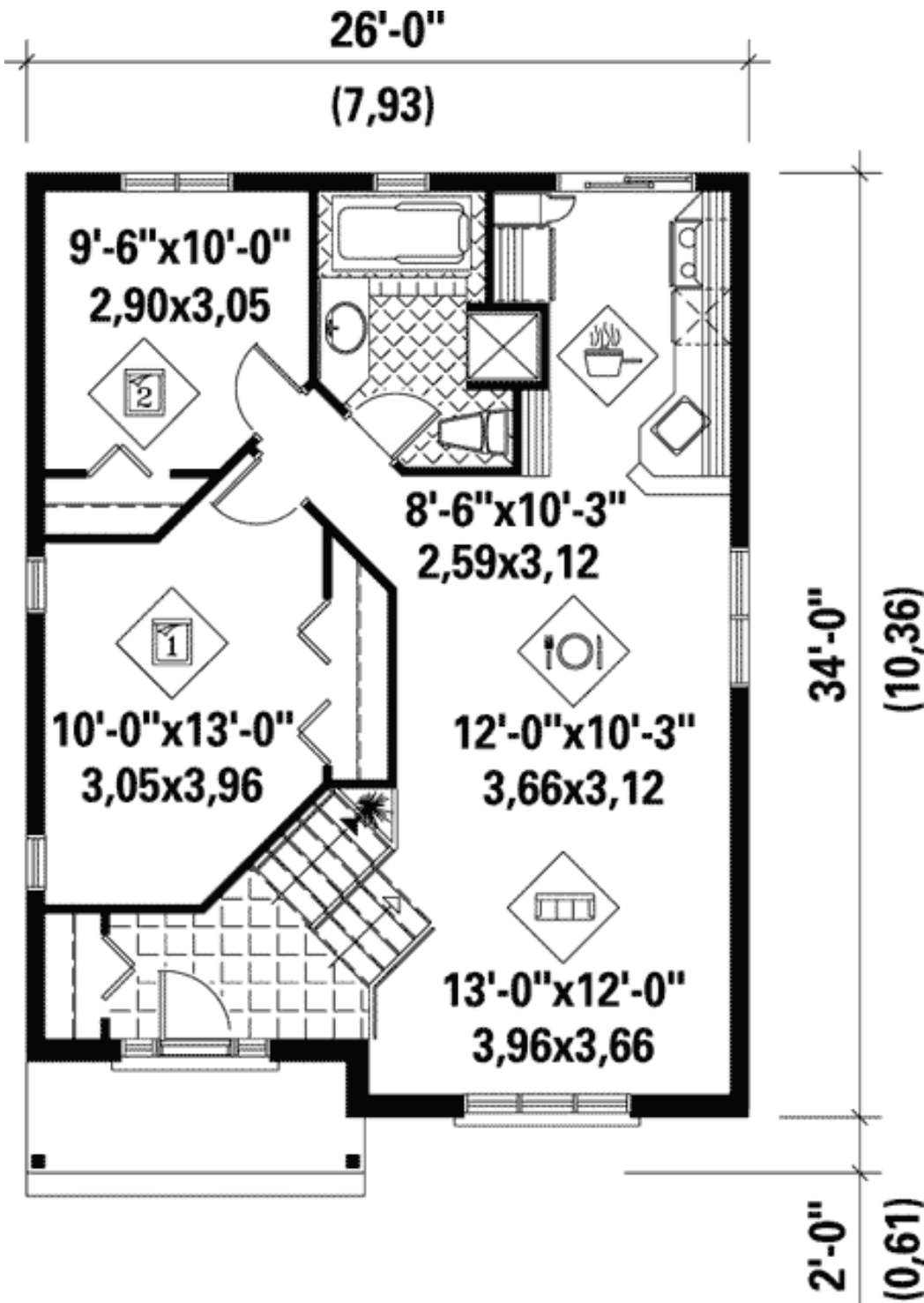
Main Level
