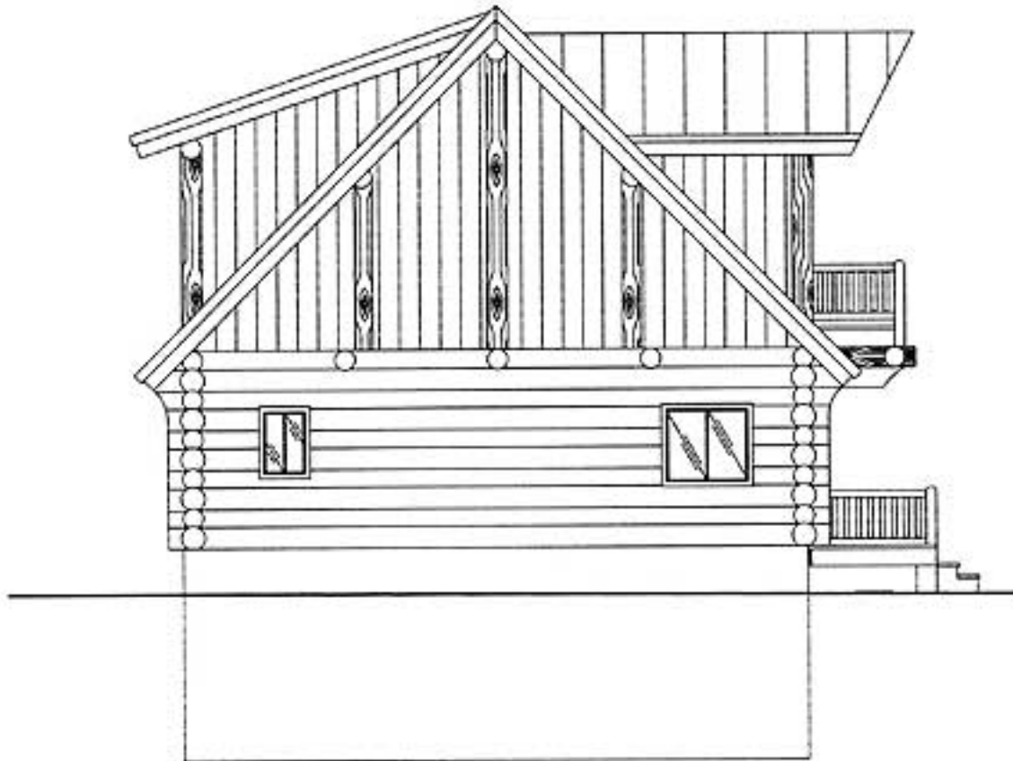
REAR ELEVATION
