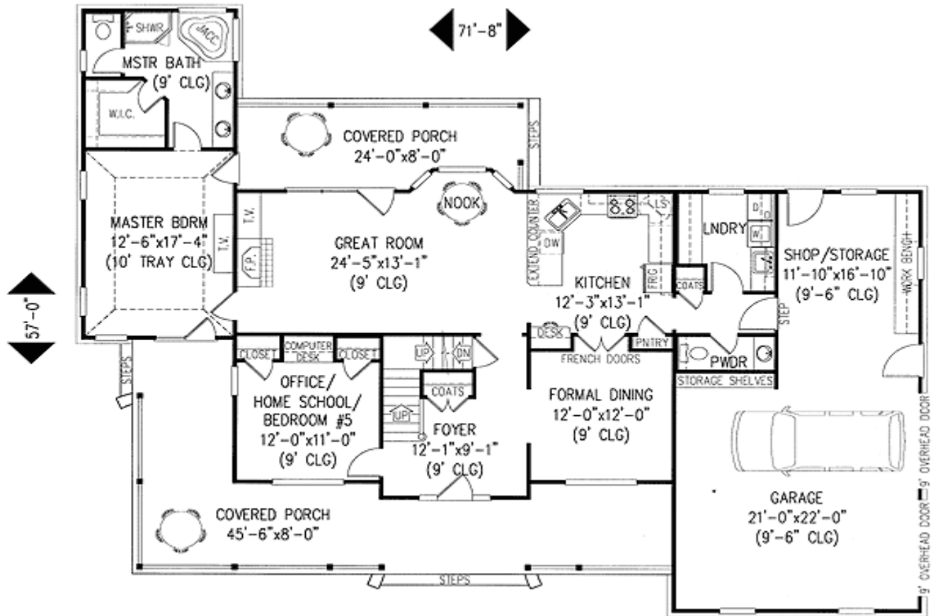
Main Level
