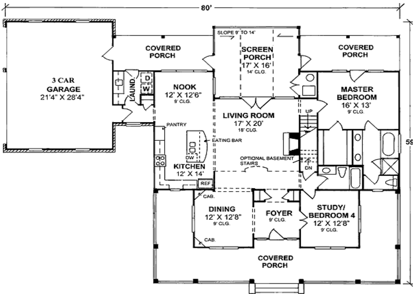
Main Level
